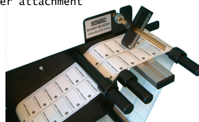
Optional 'bolt-on' label slitter attachment
